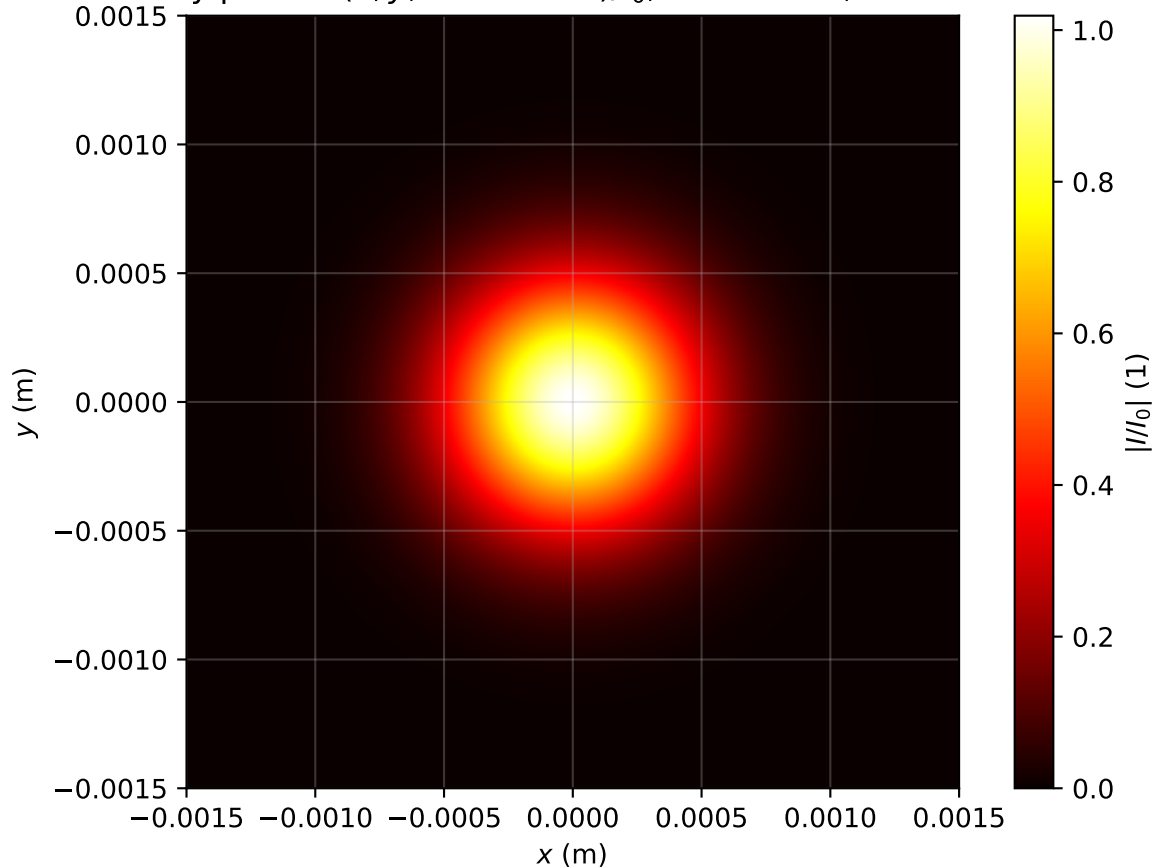
Intensity profile I(x, y, z = 0.239m)/I_0 , Pin=0.6Pcr, artificial time
